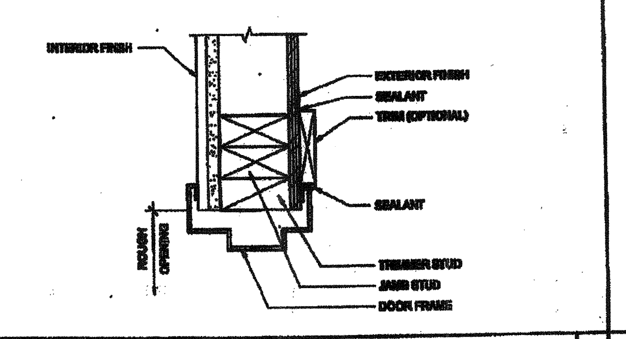
EXTERIOR DOOR JAMB SCALE: 3/4"=1'-0" 7
