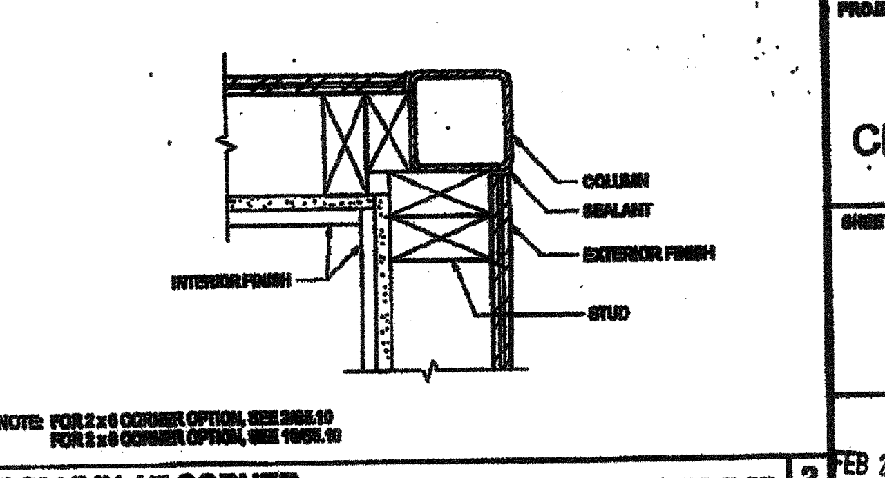
COLUMN AT CORNER SCALE: 3/4"=1'-0" 12
