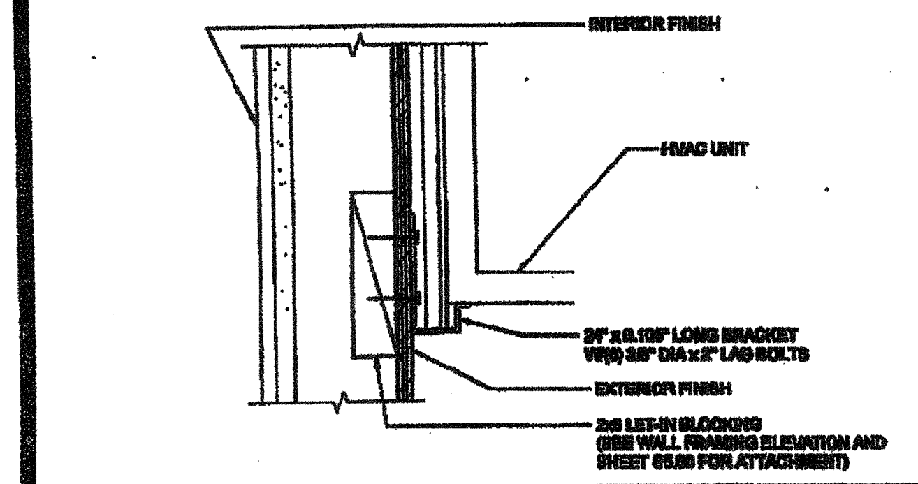
HVAC UNIT AT BOTTOM SCALE: 3/4"=1'-0" 17
