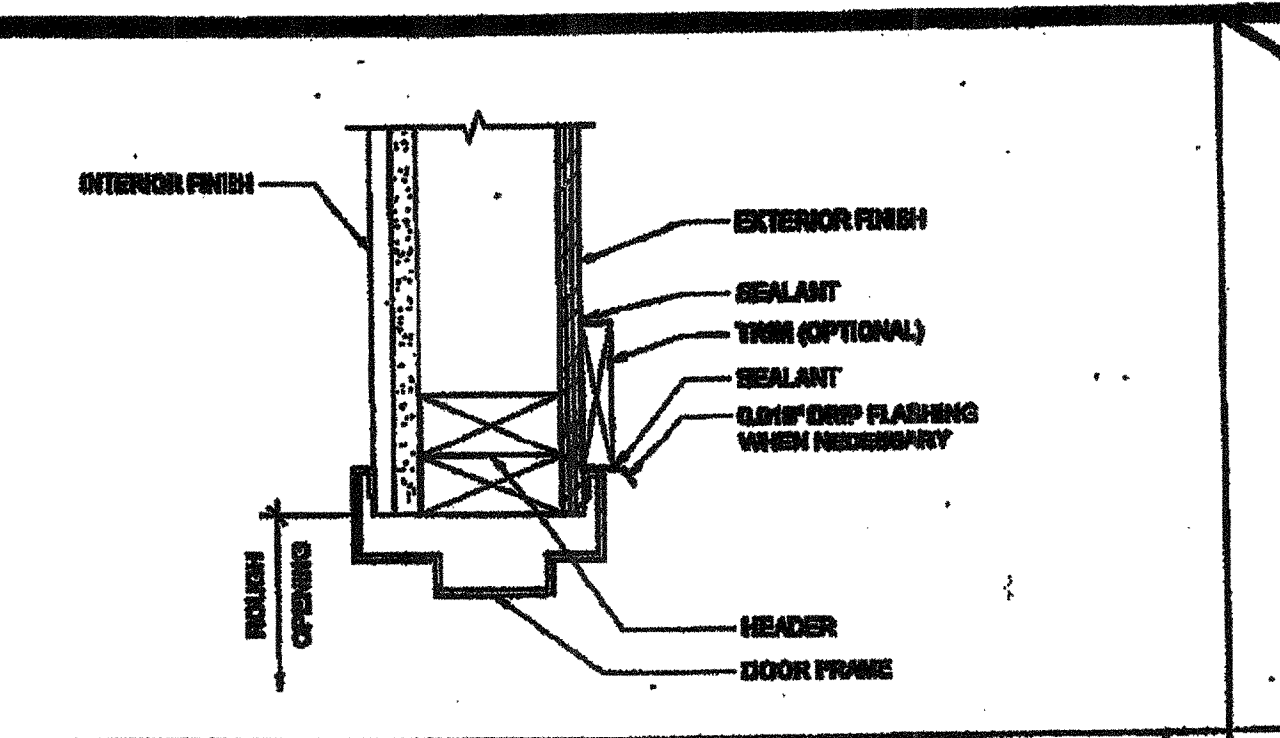
EXTERIOR DOOR HEADER SCALE: 3/4"=1'-0" 6
