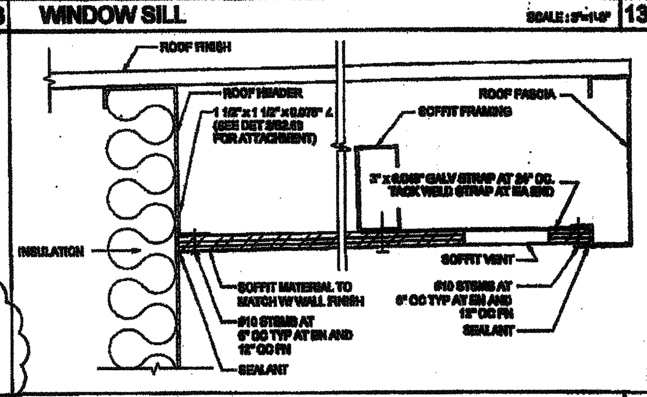
SOFFIT AT ROOF HEADER WITH VENT SCALE: 3/4"=1'-0" 14
