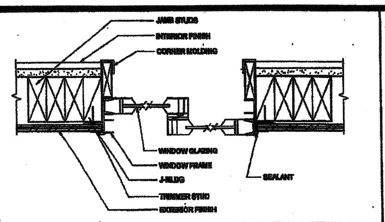
WINDOW SECTION AT JAMBS SCALE: 3/4"=1'-0" 11
