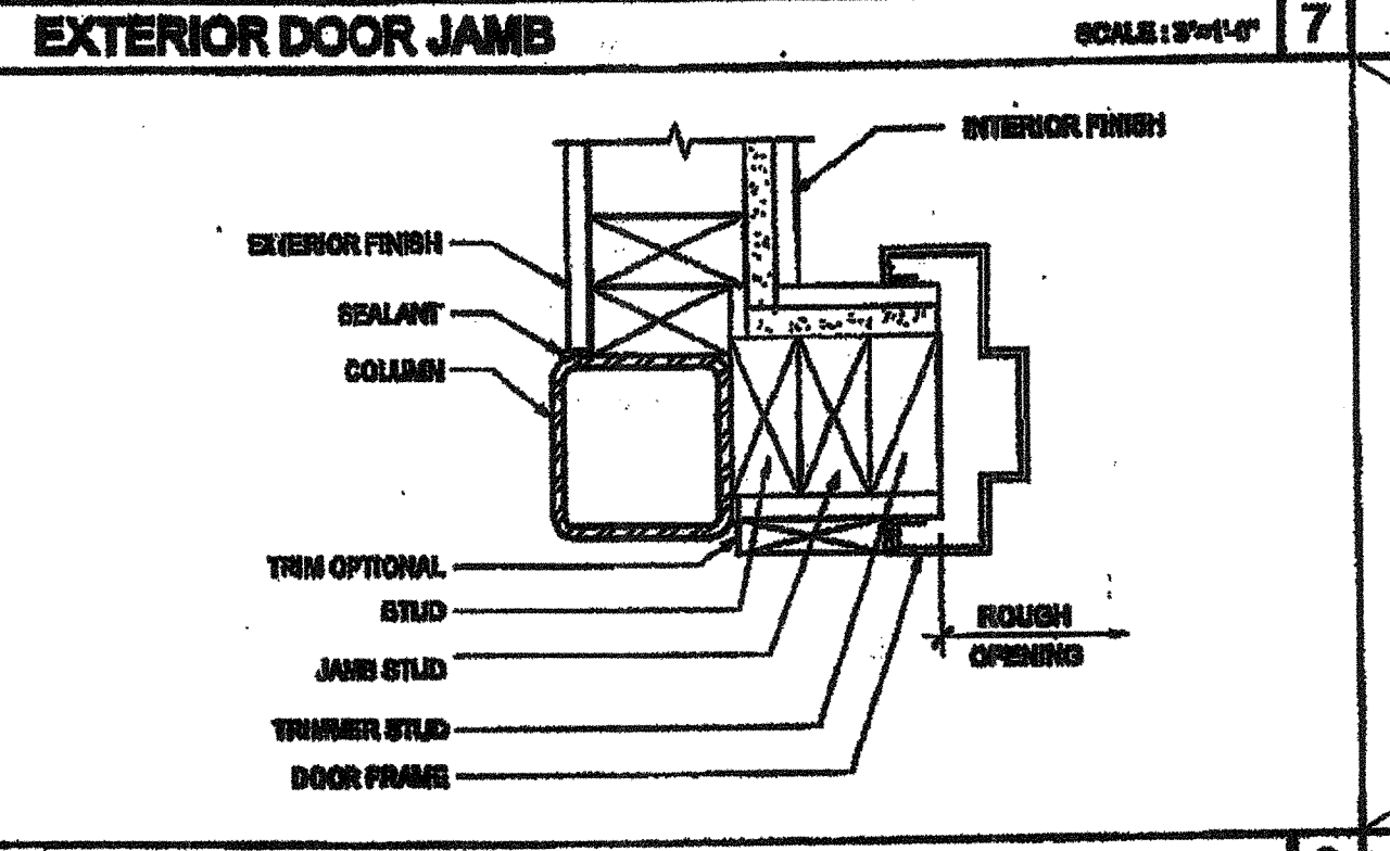
EXTERIOR DOOR JAMB SCALE: 3/4"=1'-0" 8
