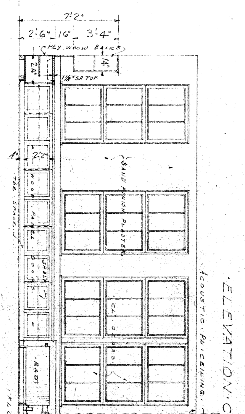
ELEVATION DETAILS OF TYPICAL CLASS ROOM.
